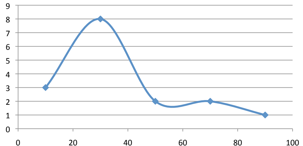
Histogram: #emails/presentation
