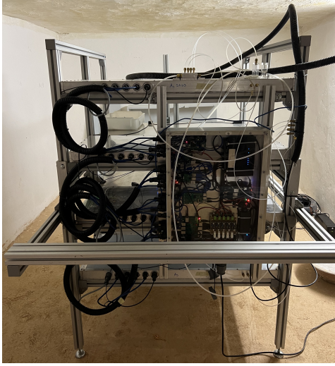
Figure 4. Front side of the detector
