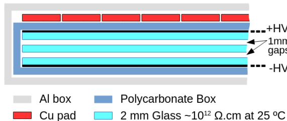
Figure 1. Schematic view of the inner components of an RPC. Adapted from [1]
