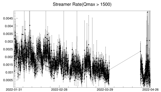
Figure 11. Streamer Rate in Coimbra(Value range: 0-1)
