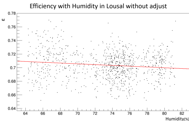
Figure 13. Correlation between efficiency and humidity in Lousal, before adjust the applied voltage, slope of the line: -5.75E - 4
