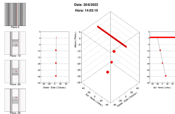
Figure 2. Determination of muon trajectories in the detector, cite from [2]
