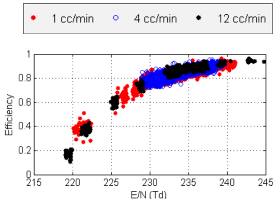
Figure 6. Correlation of efficiency with E/N , adapted from [5]
