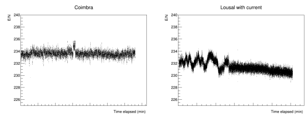
Figure 8. Comparison between the Reduced electric field variation in Coimbra and Lousal
