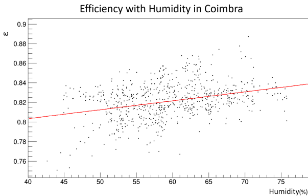
Figure 12. Correlation between efficiency and humidity in Coimbra, slope of the line: 9.13E - 4 [units?]
