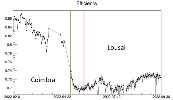
Figure 5. Variation of the efficiency along time. The detector took data in Coimbra before it was moved to Lousal in April 2022 as the green line shown. The red line represent the date we started adjust the applied voltage in Lousal, we will discuss this later.
