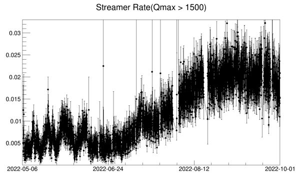
Figure 10. Streamer Rate in Lousal(Value range: 0-1)
