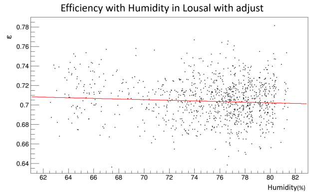
Figure 14. Correlation between efficiency and humidity in Lousal, after adjust the applied voltage, slope of the line: -3.27E - 4
